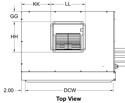
Figure 43: Vertical Unit Dimensions (Unit Sizes 030-050)
