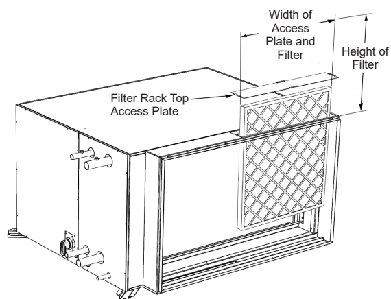
Top Filter Access Clearance Cabinet Sizes: 030 – 050
