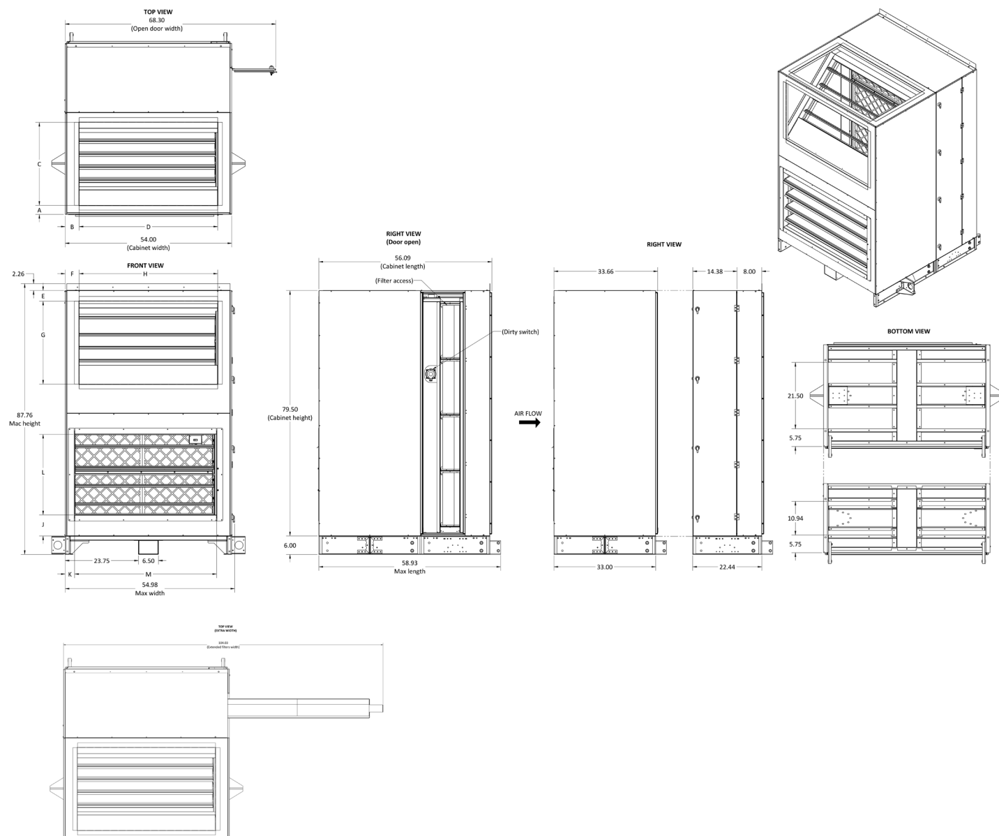
Figure 60: Vertical Economizer End Section Dimensions (Unit Sizes 060-100)
