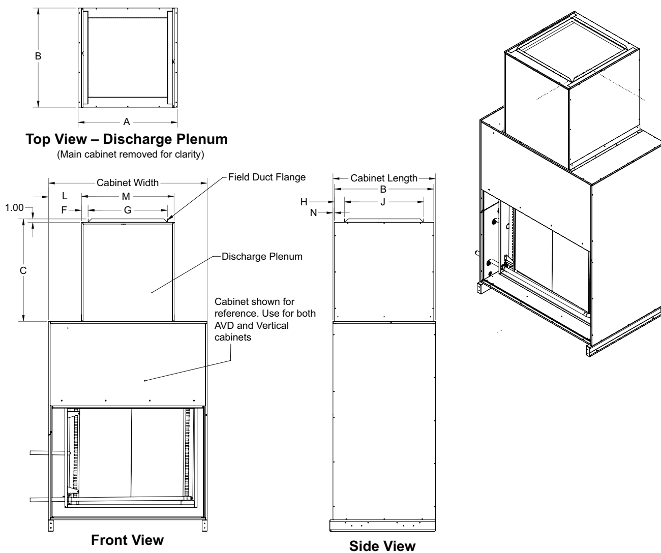
Figure 45: Vertical Discharge Plenum (Unit Sizes 006-050)
