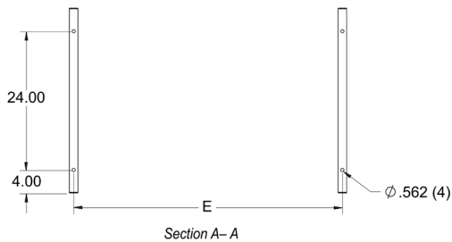
Cabinet Mounting Hole Locations
