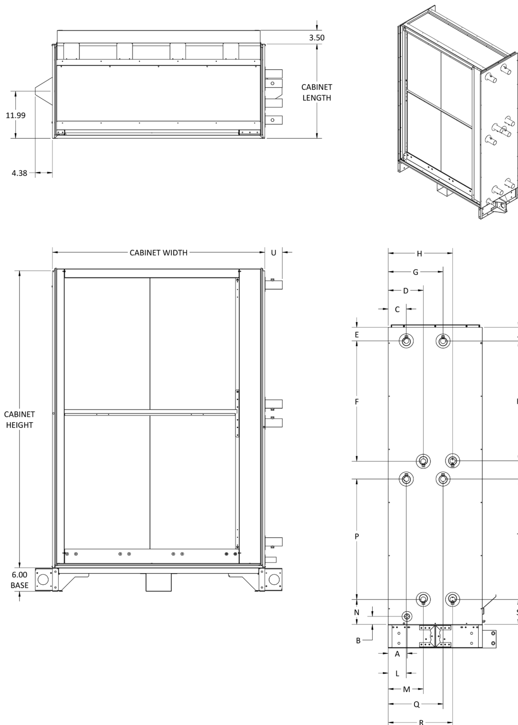
Figure 48: Vertical Hydronic Coil Unit Dimensions (Unit Sizes 060-100)
