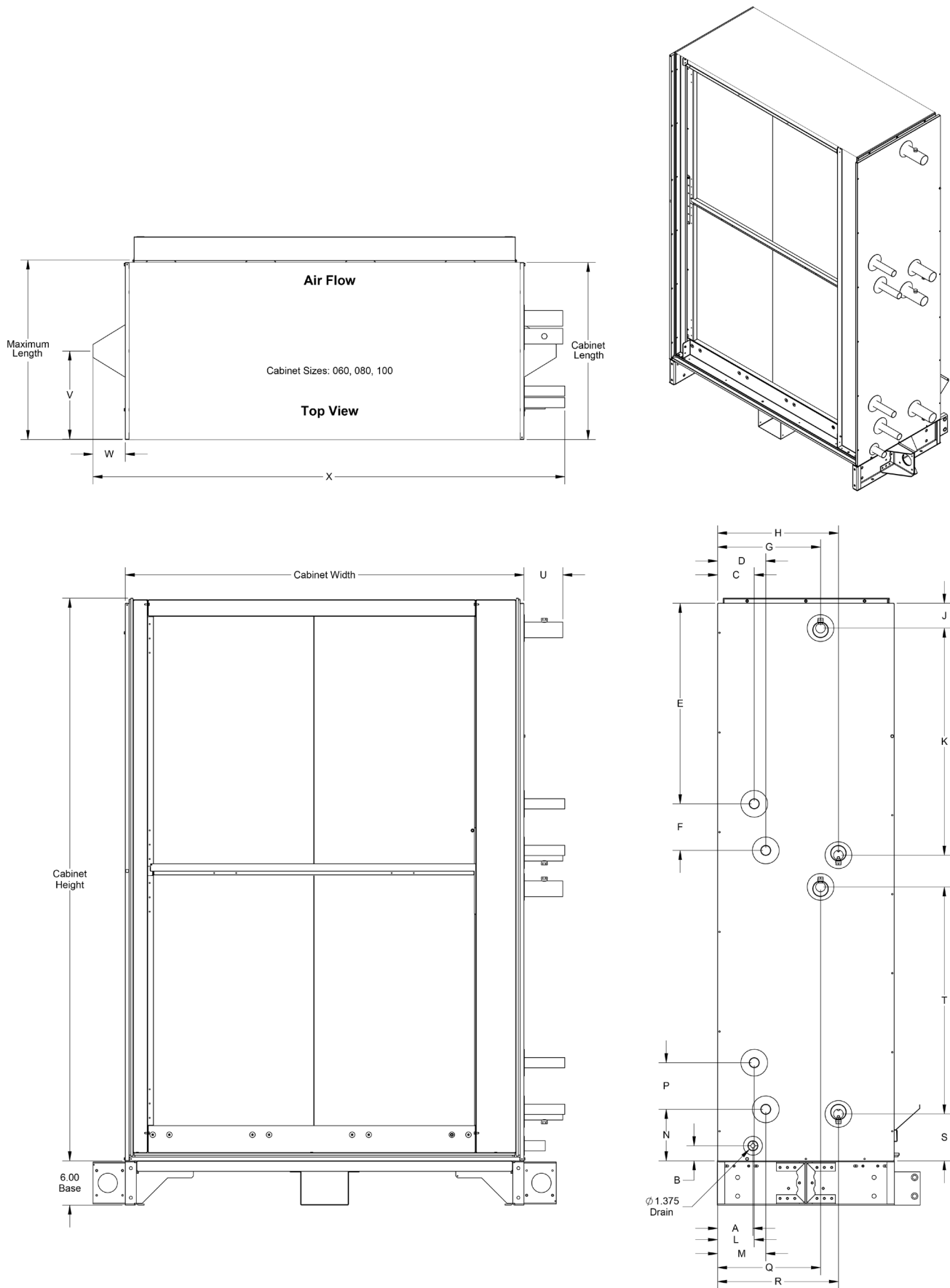
Figure 49: Vertical Unit DX Coil Dimensions (Unit Sizes 060-100)
