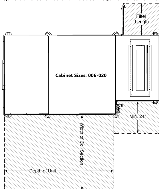
Figure 68: Clearance and Access Requirements for Horizontal Units (Unit Sizes 006-050)
